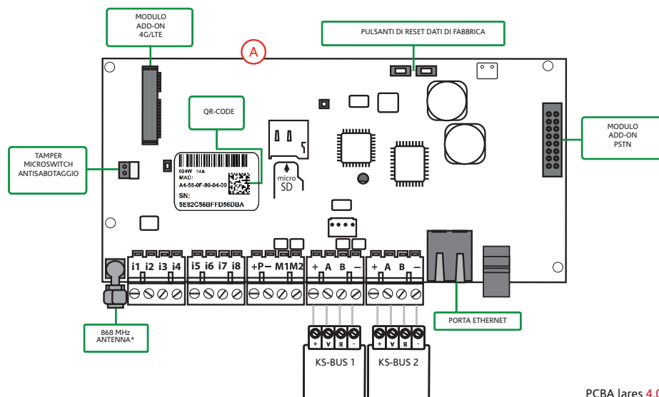
PCBA lares 4.0
